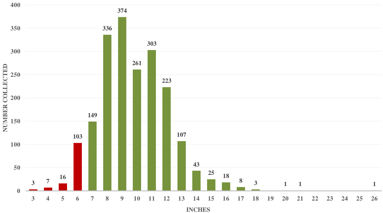
2022 Brown Trout Sizes Upper Smith River (N=1980)
