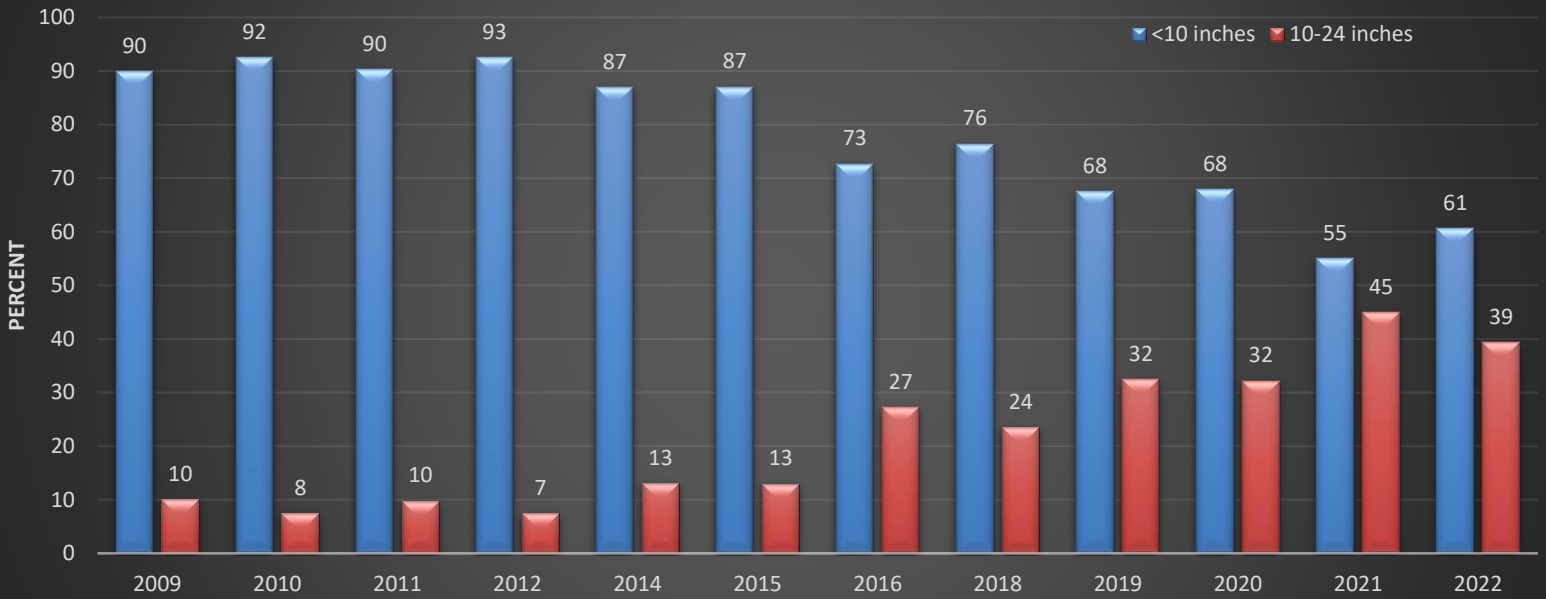
Percent of Brown Trout Collected smaller than 10" & 10-24" (2009-2022)
