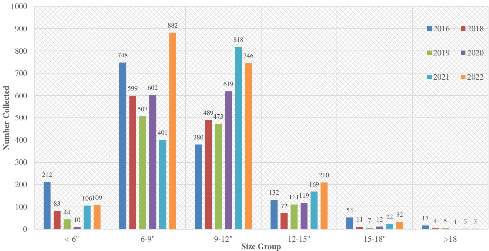
Number of Brown Trout Collected by Size Group (2016-2022)
